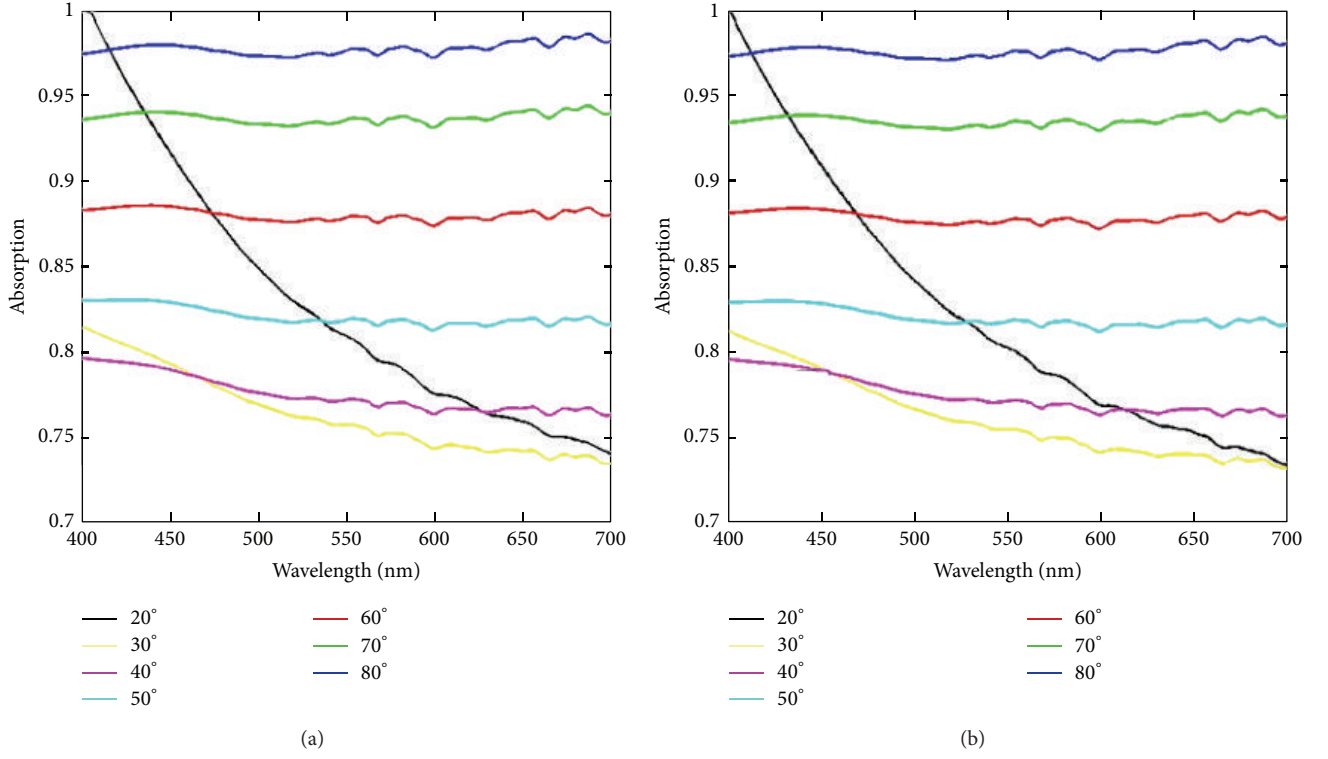
FIGURE 3: Absorptive spectra of quadrangular frustum pyramid array under various angle. (a) For different incident angles from 20° to 80°. (b) For different incident angles from 20° to 80°.
