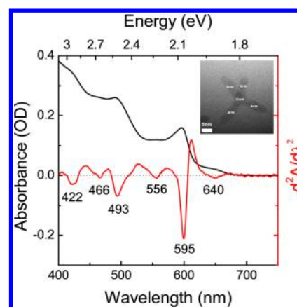
Figure 1. Steady-state absorption spectrum (black line) of tetrapod-shaped CdSe NCs. The second derivative of the broad absorption spectrum is shown by a red line. The inset shows TEM images of tetrapod-shaped CdSe NCs (denoted as core/arms) prepared by the seeded-growth approach.
