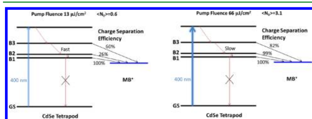
Figure 5. Schematic diagram of charge separation processes from different energy levels of CdSe tetrapod to MB + molecule under low (left) and high (right) pump fluences. B1, B2, and B3 are the assigned absorption bands in Figure 2b. GS is the ground state. Blue solid arrows, red dot arrows, red solid arrows, and black solid arrows represent excitation, relaxation, radiative recombination, and charge separation processes, respectively.
