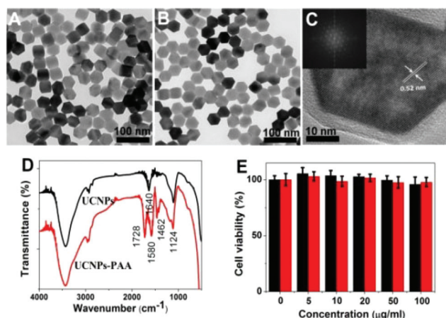
Fig. 2 (A) TEM image of ligand free NaYF 4 :Yb 3+ ,Er 3+ UCNP. (B) PAA coated UCNP. (C) TEM image of a single nanoparticle, with the corresponding diffractogram (inset). (D) FTIR spectra of ligand free UCNP and PAA coated UCNP. (E) Cellular viability results based on the standard MTT assay.
