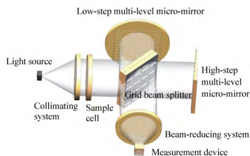
Fig.1 Schematic diagram of the static and light FTIR
