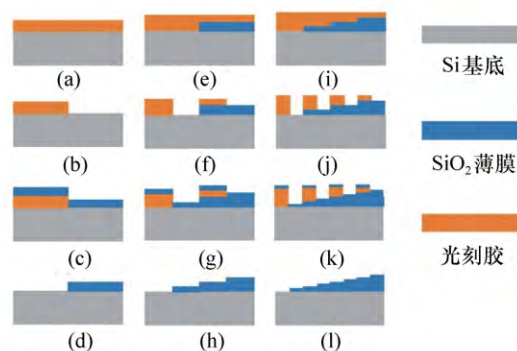
Fig.4 Flow diagram of low-stepped multi-level micromirrors (with 8 steps as an example)
