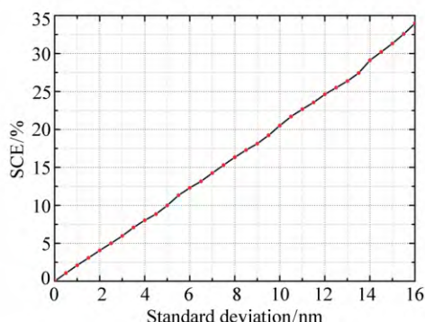
Fig.3 SCE varies with height standard deviation \sigma of the sub-mirror
