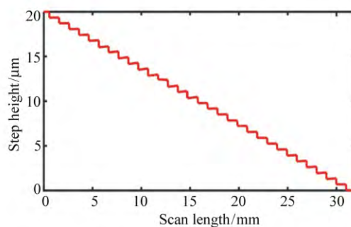
Fig.8 Step height test results of low stepped micromirror with 32 steps
