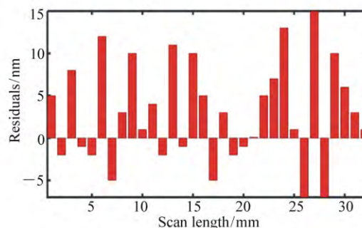
Fig.9 Step height difference between the measured values and their theoretical values
