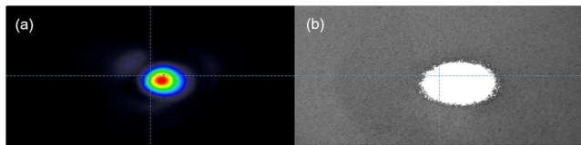
Fig. 2. Nd:YAG laser beam position at the wavelength of 355 nm with 0.5 \text{ J/cm}^2 laser peak fluence in (a) the beam profiler and (b) the CCD camera. The silver film was tested for beam position calibration.
