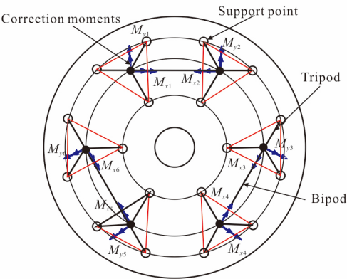
图 2 2 m SiC 轻量化主镜支撑方案简图 Fig.2 Support program diagram of 2 m SiC lightweight primary mirror
