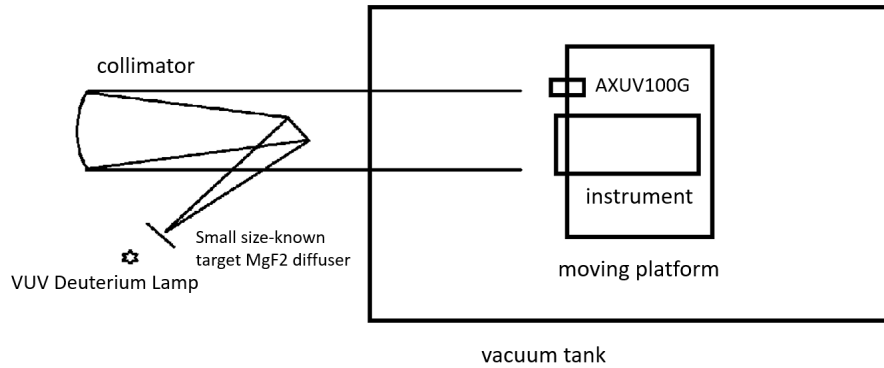
Fig. 21 Schematic diagram of radiometric response calibration at 121.6 nm.
