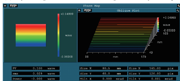
(c) 调整垫安装面倾角面型等效结果 (c) Equivalent result of inclination surface of adjustable pad mounting surface
