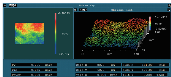
(b) 调整垫安装平面的倾角面型检测结果 (b) Adjusted angle of face surface of mounting surface of adjustable pad
