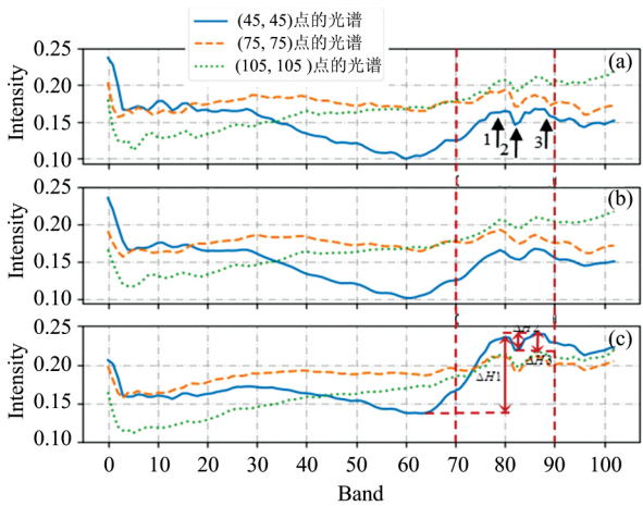
图 5 采用不同滤波算法后的光谱 (a): 原始光谱; (b): SG 滤波后光谱; (c): TSG 滤波后光谱 Fig 5 The spectrum after processed by different filtering algorithms (a): Raw spectrum; (b): Processed by SG filter; (c): Processed by TSG filter
