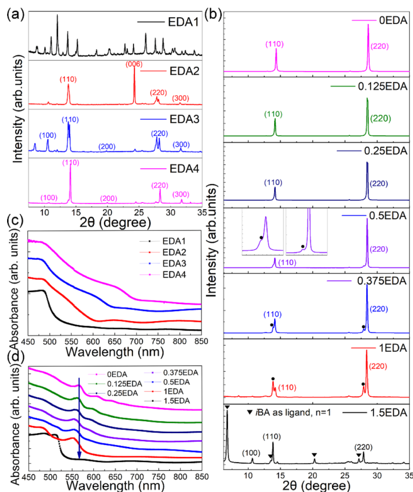
Figure 2. (a) XRD spectra of the thin-film samples of \text{EDA}(\text{MA})_{n-1}\text{PbI}_{3n+1} . When n varies from 1 to 4, they stand for the samples of EDA1, EDA2, EDA3, and EDA4 (Group 1 samples). (b) XRD patterns of the thin-film samples of (\text{iBA})_2(\text{MA})_{3-2x}(\text{EDA})_x\text{PbI}_{13} . As x changes from 0 to 1.5, they refer to the samples of 0EDA, 0.125EDA, 0.25EDA, 0.375EDA, 0.5EDA, 1EDA, and 1.5EDA, accordingly (Group 2 samples). (c) Absorption spectra of Group 1 samples. (d) Absorption spectra of Group 2 samples.
