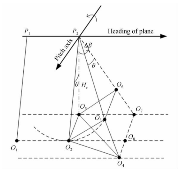
图 5 俯仰角变化对重叠率影响 Fig. 5 Effect of pitch variation for overlap
