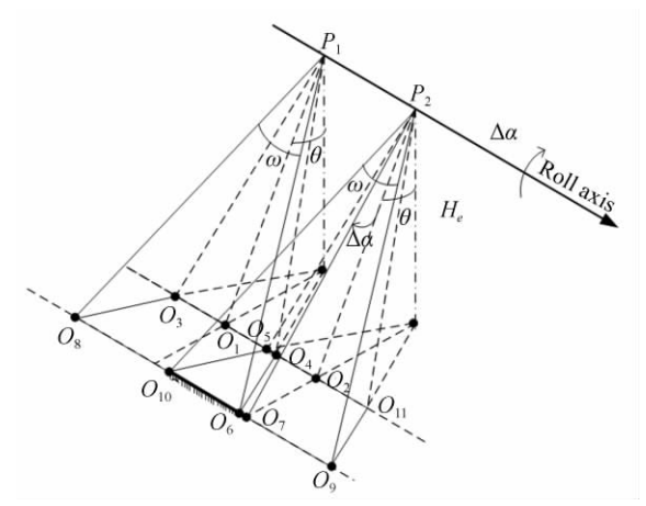
图 6 横滚角变化对重叠率影响 Fig. 6 Effect of roll variation on overlap
