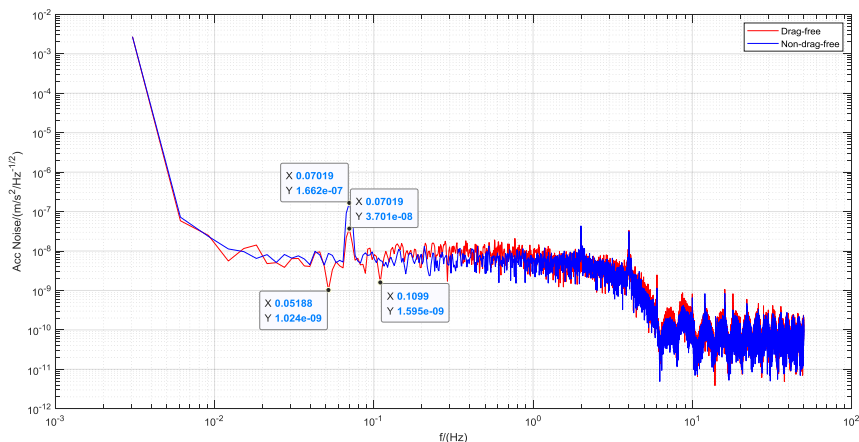
Fig. 12. (Color online) ASD spectra of the GRS acceleration measurements along the earth-center direction under 0.07Hz disturbance with and without drag-free control (blue line: only disturbance injection; red line: disturbance injection and drag-free control).
