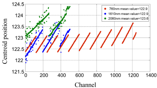
Fig. 12. The centroid positions of the slit that measured by the three spectrometers. Red line represents the 0.76 \mu\text{m} band, blue line represents the 1.61 \mu\text{m} band, and green line represents the 2.06 \mu\text{m} band (For interpretation of the references to colour in this figure legend, the reader is referred to the web version of this article).
