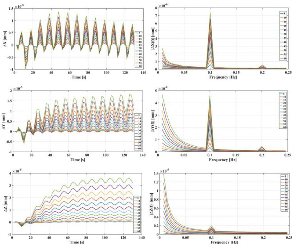
Fig. 7. Left: The displacement change curves of the node-2 in the X, Y, Z directions with time, under different temperature amplitudes of the heat source. Right: The amplitude spectrum curves after the fast Fourier transform of the displacement data (since the response amplitude is too big at 0 Hz, it is not shown in the plot).
