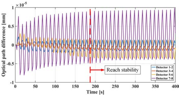
Fig. 12. (Color online) When the heat source temperature amplitude is 10 K, the time-domain response curves of the interference arm length difference for each interferometer (simulation time: 400 s), and the red dotted line presents the estimated time to reach stable.
