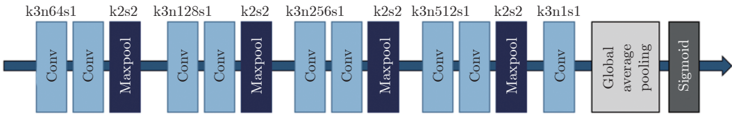
图 14 NMD 结构 [45] Fig.14 The NMD structure [45]
