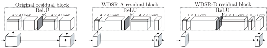
图 12 三种残差模块的对比 [41] Fig.12 Comparison of three residual blocks [41]
