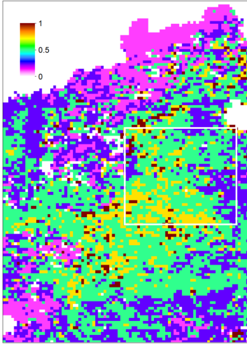
(c)201905 AOD_f\_aver
