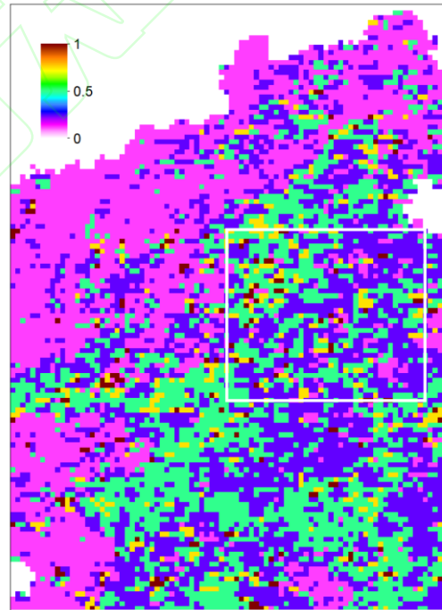
(f)201908 AOD_f\_aver
