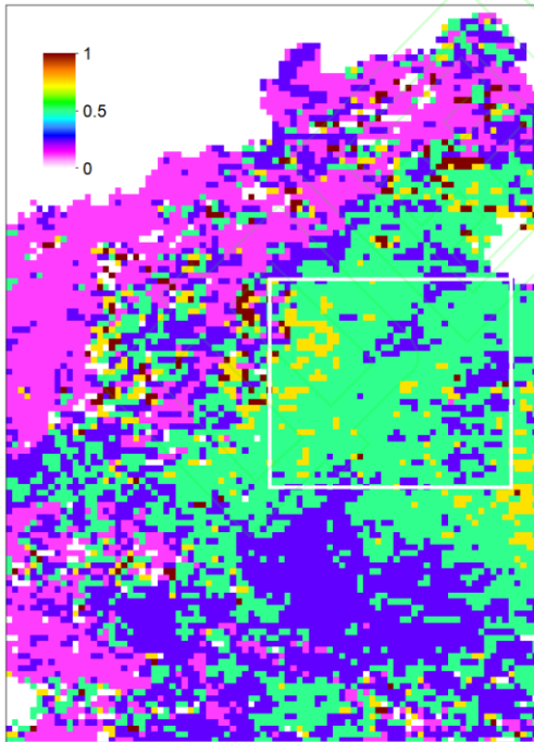
(e)201907 AOD_f\_aver
