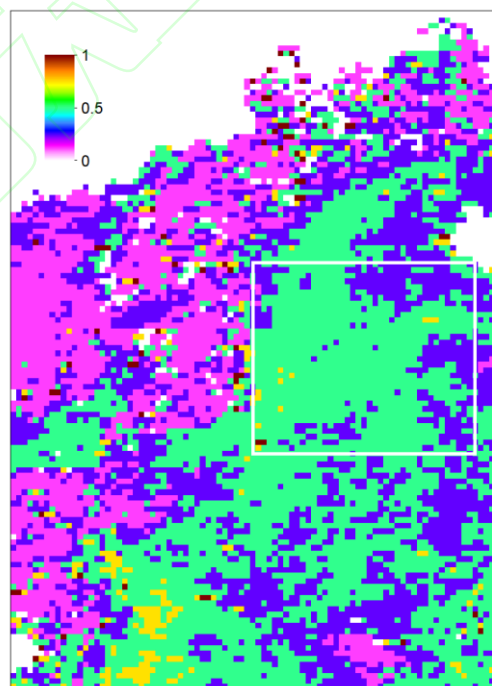
(n)201912 AOD_f\_aver
