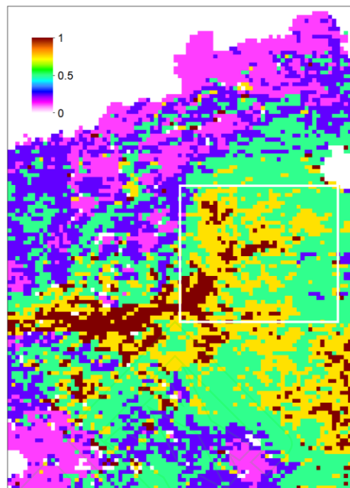
(h)201910 AOD_f\_aver
