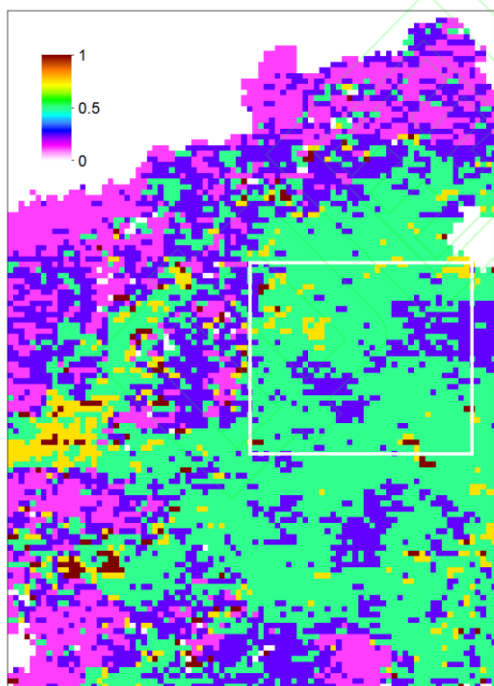
(m)201911 AOD_f\_aver
