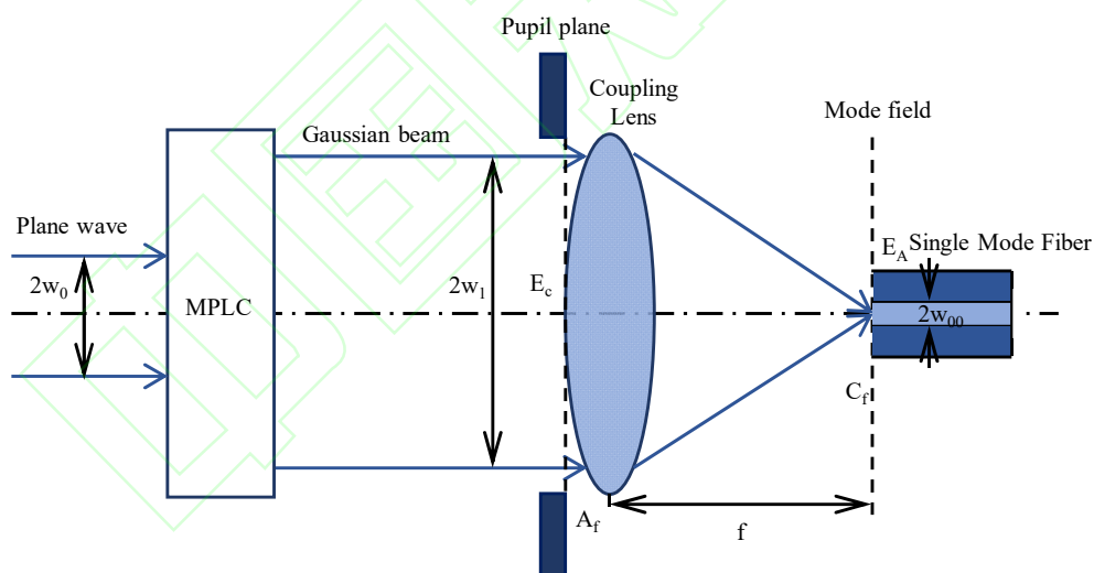
Fig.6 Schematic diagram of spatial optical - single-mode fiber based on MPLC
