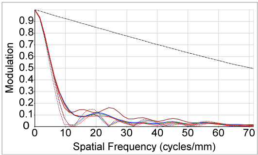
图 10 支撑结构为高体份的 MTF 曲线 Fig.10 MTF curves of SiCp/AL-HT8 support structure
