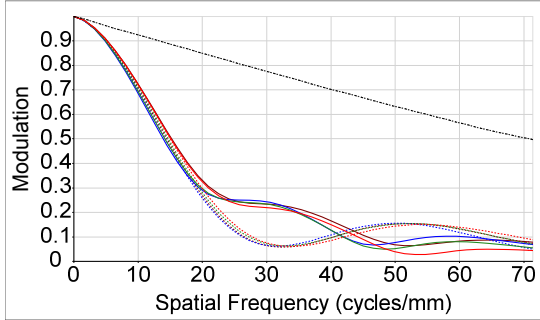
图 11 支撑结构为钛合金的 MTF 曲线 Fig.11 MTF curves of TC4 support structure
