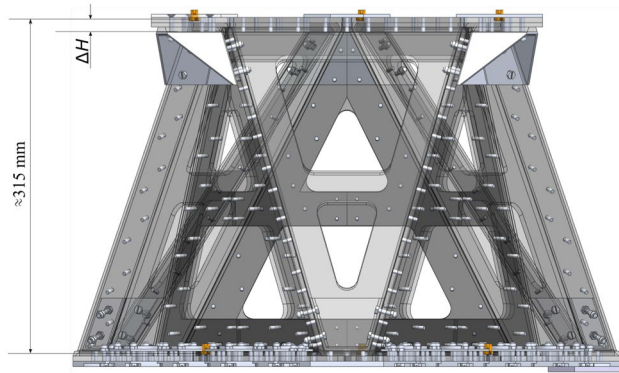
Fig. 13 The CAD model of the C/SiC supporting frame, and \Delta H is the transverse thickness of the C/SiC plate
