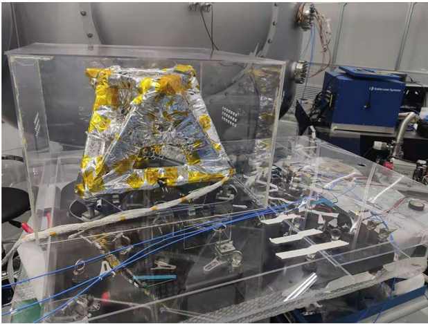
Fig. 5 The experimental scene of the thermal deformation measurement interferometry system
