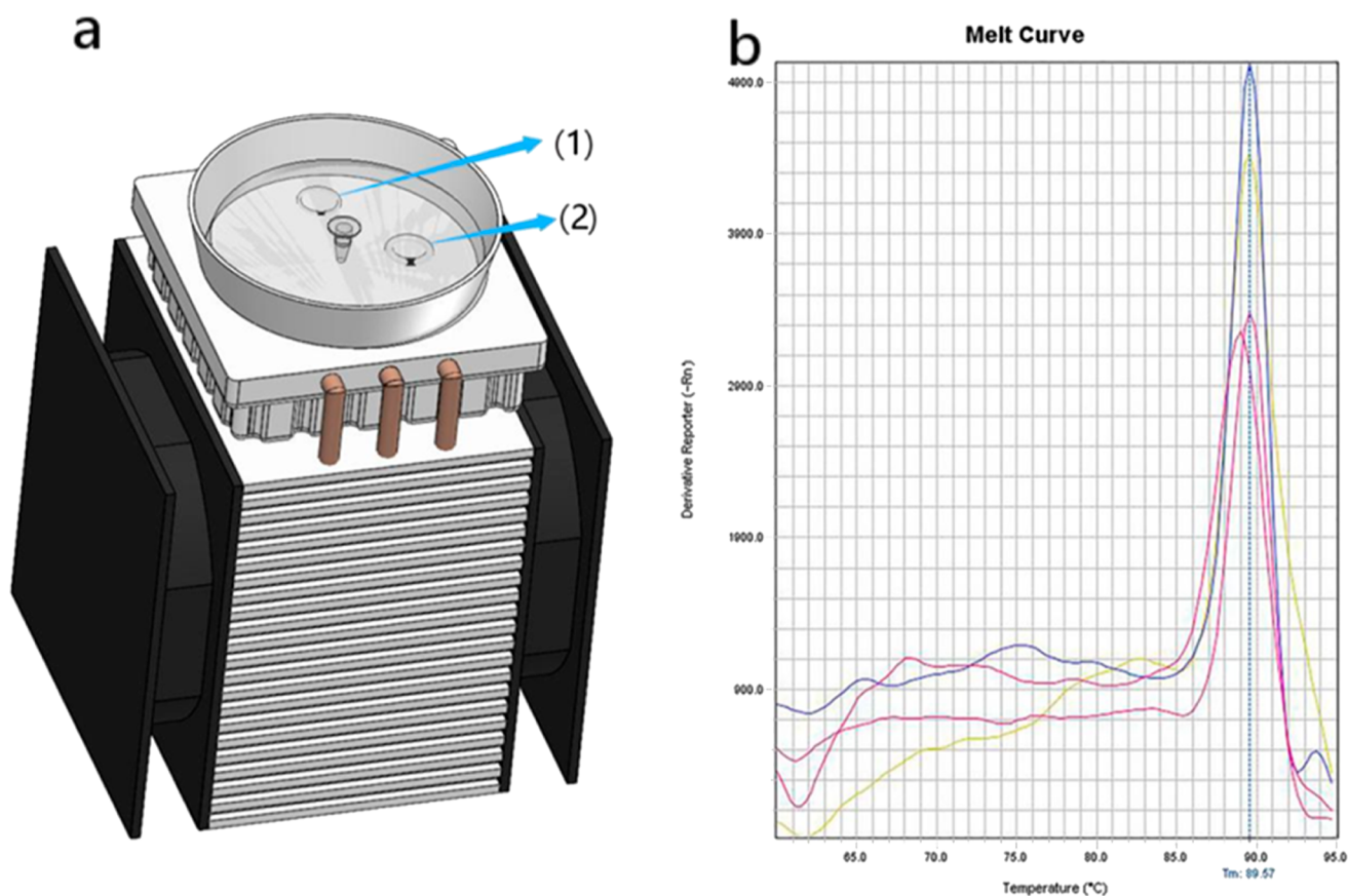
Figure 6. Experimental equipment diagram (a). A PCR tube and two ring-shaped Teflon tubes with different inner and outer diameters are placed in a liquid metal bath, using a commercial qPCR cyclers as a reference. Comparison of the melting curves of the four groups of experiments (b).
