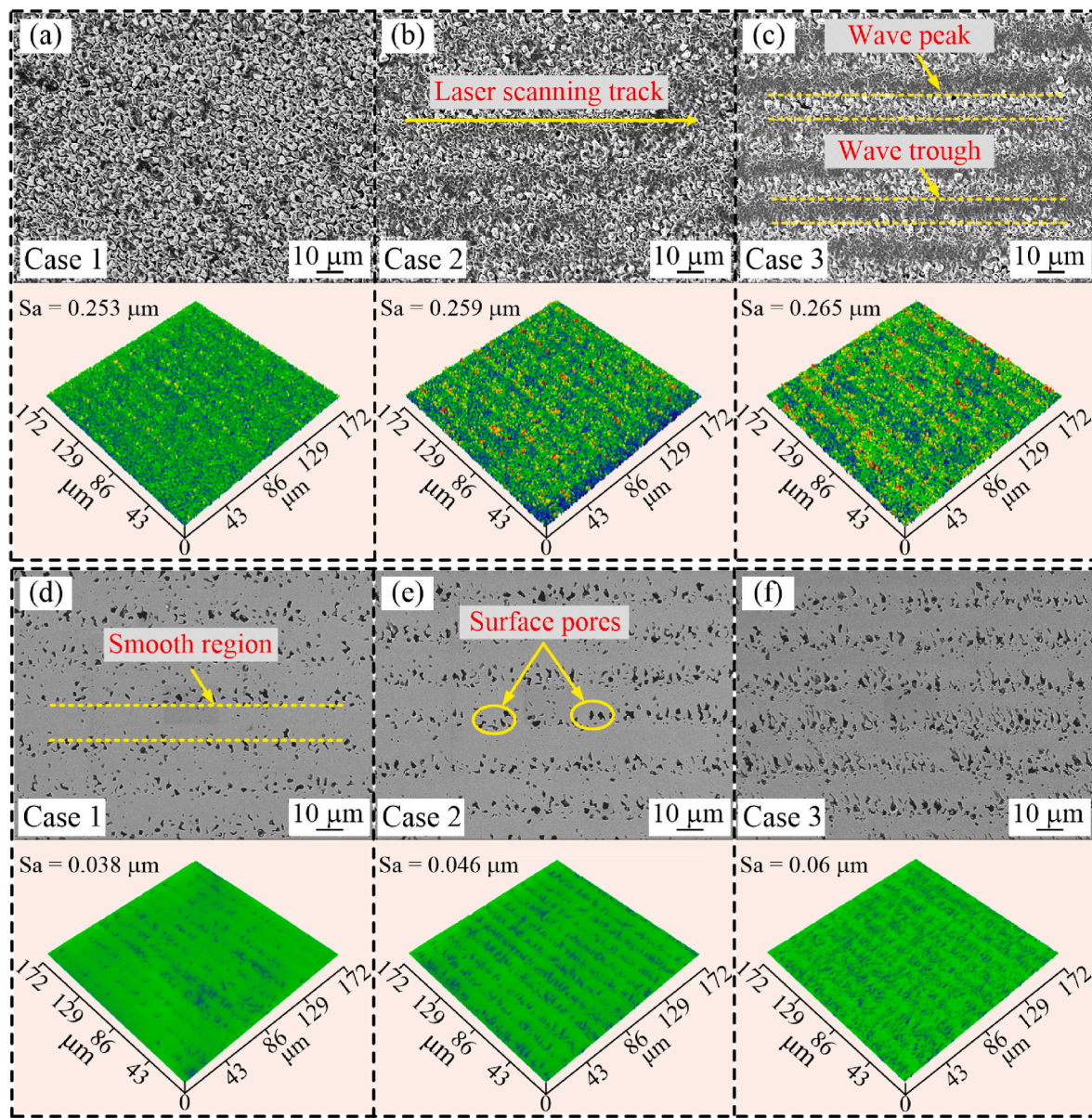
Fig. 3. SEM micrographs and 3D topographies of the laser nitrided surfaces: (a) case 1, (b) case 2, and (c) case 3. SEM micrographs and 3D topographies of the laser nitrided surfaces after mechanical polishing: (d) case 1, (e) case 2, and (f) case 3.
