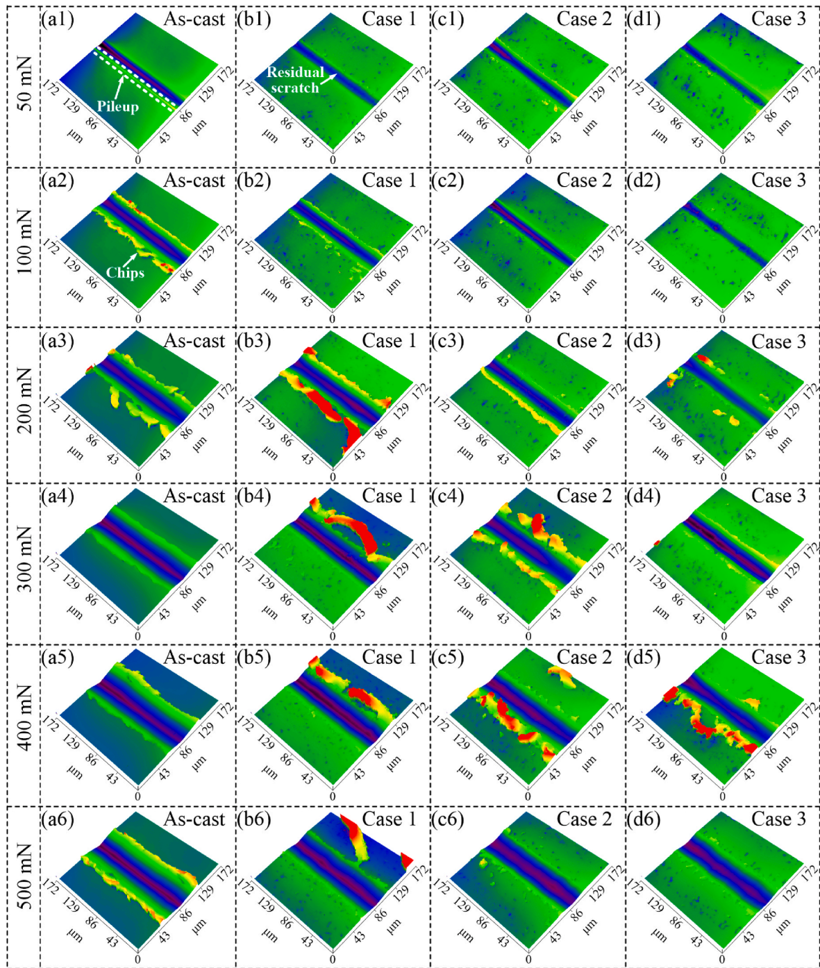
Fig. 6. 3D topographies of the residual scratches on the as-cast MG and cases 1–3 surfaces under various normal loads.
