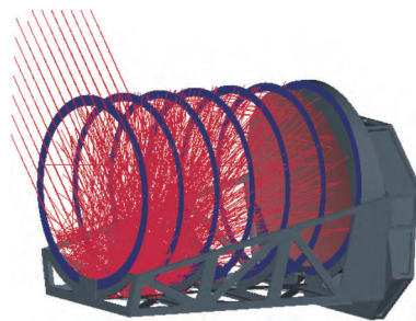
图8 空间引力波望远镜追迹示意图 Fig. 8 Ray-tracing diagram of the spaceborne gravitational wave telescope
