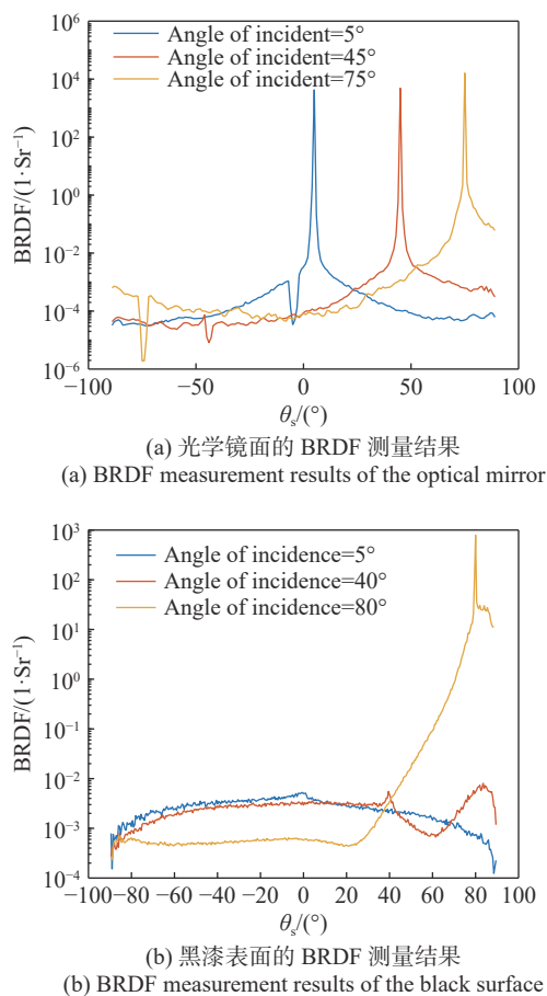
Fig. 7 Scattering measurement results of the scattering surface
