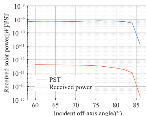
图9 空间引力波望远镜 PST 与接收到的杂散光功率 Fig. 9 The PST and the received stray light powers of the spaceborne gravitational wave telescope
