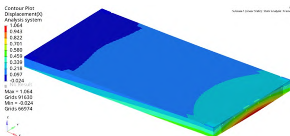
Fig. 17 Contour plot of X -direction displacement
