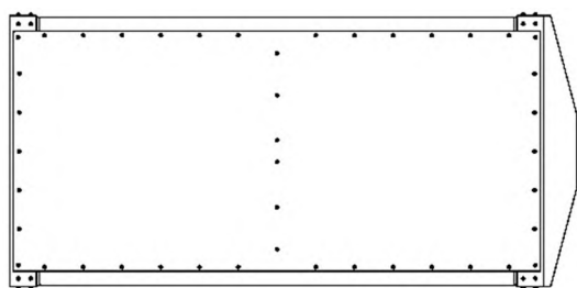
Fig. 12 Distribution of skin-frame bolts with half the number
