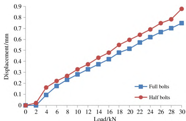
Fig. 13 Displacement curves of point 2 with different numbers of skin-frame bolts
