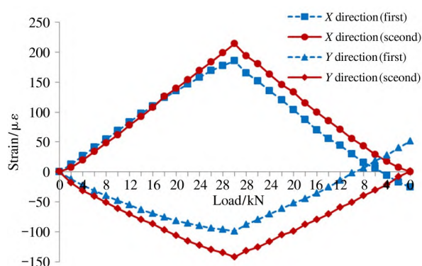
Fig. 7 Strain curves of point Y8 in composite structure
