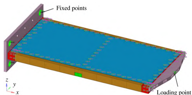
Fig. 14 Finite element model of the composite structure
