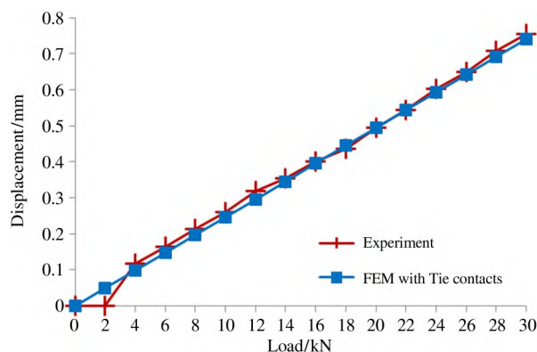
Fig. 22 Displacement curves of point 2 with Tie contacts
