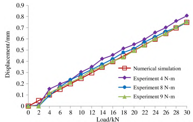
Fig. 19 Displacement curves of point 2 with comparison of simulation and experimental results
