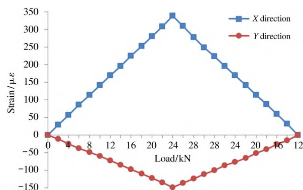
Fig. 10 Strain curves of point Y13 in frame
