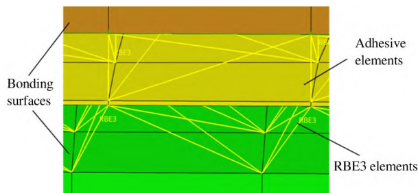
Fig. 16 Modeling of adhesive connection
