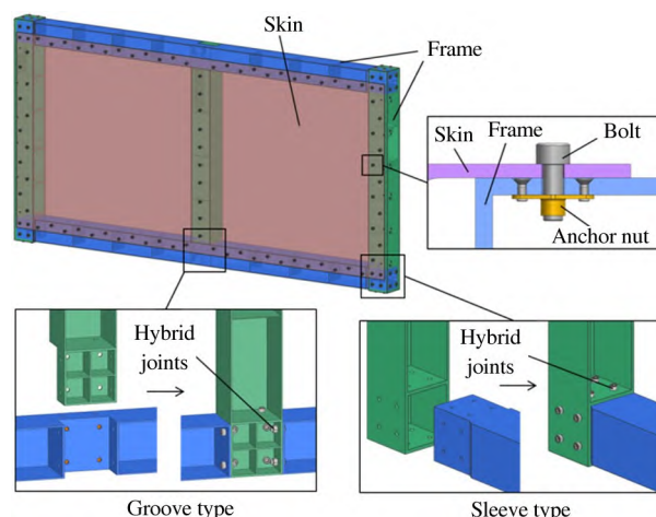
Fig. 1 Composite structure with multi hybrid joints
