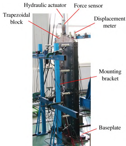
Fig. 3 Test stand of the composite structure
