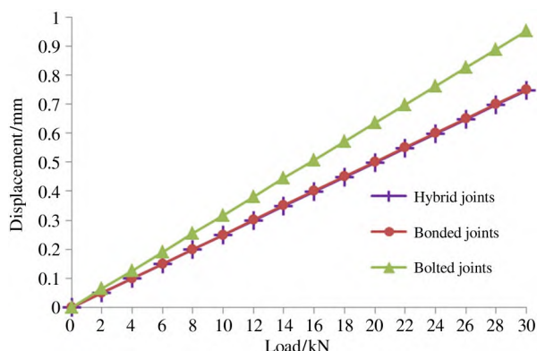
Fig. 20 Displacement curves of point 2 with different joints
