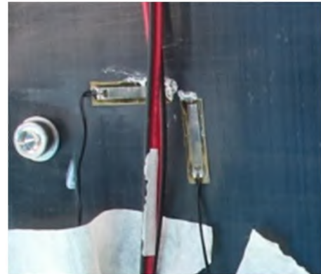
Fig. 5 Cross strain gauges used
