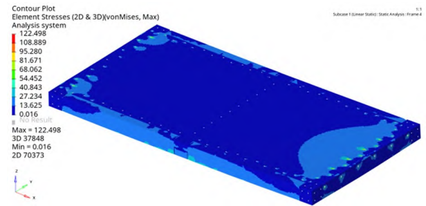
Fig. 18 Contour plot of element stresses
