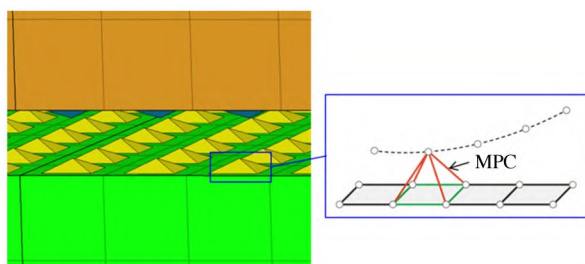
Fig. 21 Tie contacts in finite element model
