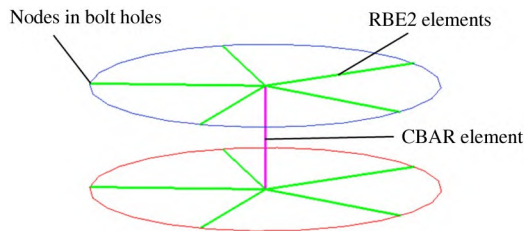
Fig. 15 Modeling of bolted connection
