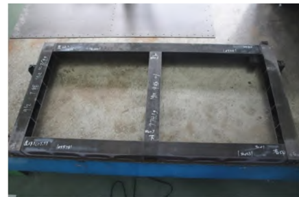
(a) Assembly of frame before bonding
