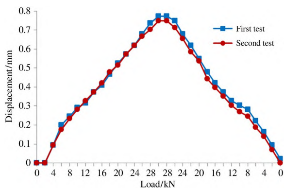
Fig. 6 Displacement curves of point 2 in composite structure
