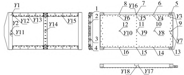
Fig. 4 Distribution of measurement points
