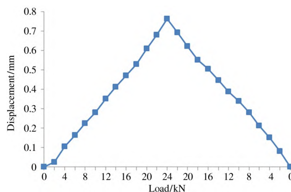
Fig. 9 Displacement curve of point 2 in frame
