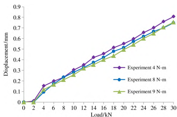
Fig. 11 Displacement curves of point 2 with different tightening torques of skin-frame bolts
