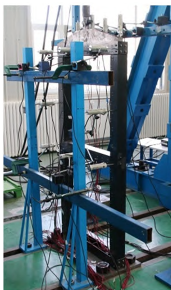
Fig. 8 Tensile test of the frame only
