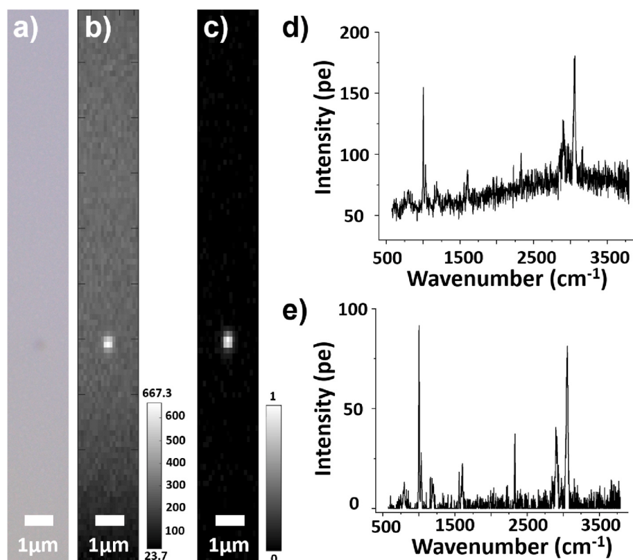
Fig. 4. Results for a 200 nm PS bead using the 0.95NA dry objective. A) Reflection image. B) Line scan Raman image of the 3055- 3062 \text{cm}^{-1} peak area. C) PS chemical component concentration image of the region in (a) after FSC 3 analysis. D) Spectrum at bead center. E) PS component spectrum.
