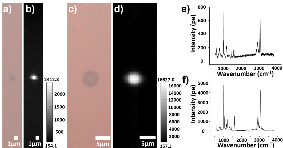
Fig. 2. Spatial imaging of PS beads using the 0.6 NA dry objective. a) Reflection image of a 1 \mu\text{m} bead and b) corresponding line-scan Raman image of the peak area over 3055–3062 \text{cm}^{-1} using 200 nm step size. c) and d) - as a) and b) for a 5 \mu\text{m} bead using 500 nm step size. e) and f) spectrum centered at the 1 \mu\text{m} and 5 \mu\text{m} PS bead, respectively. Data were taken with 120 mW at the sample and 1 s exposure time. Gray scale as shown.
