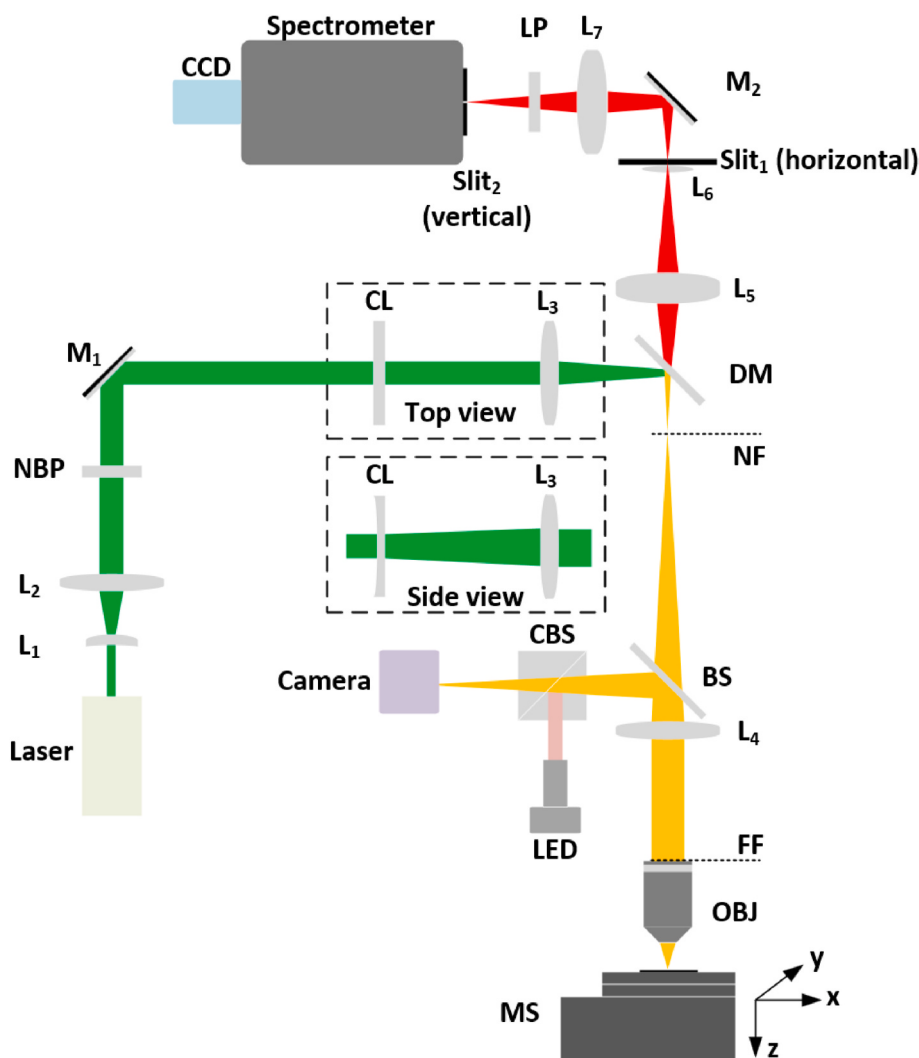
Fig. 1. Sketch of the confocal line-scan Raman spectroscopy setup. L1 to L7 – lenses, NBP – narrow band pass filter, M1 and M2 – mirrors, CL – cylindrical lens, DM – dichroic mirror, BS – beam splitter, CBS – cube beam splitter, OBJ – objective lens, MS – motorized stage, LP – long pass filter, NF – near field image plane, FF – far field image plane.
