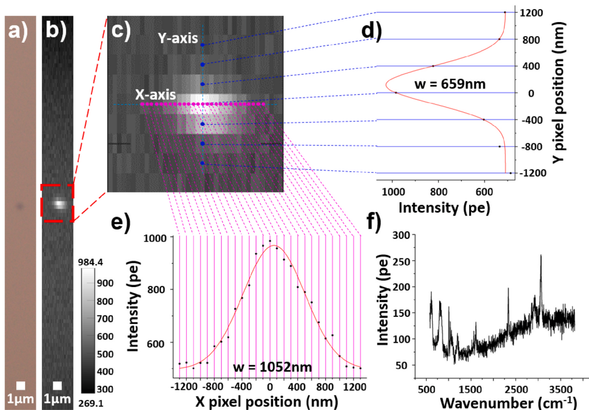
Fig. 3. Raman imaging of a 500 nm PS bead using the 0.6 NA dry objective. a) Reflection image. b) Line scan Raman image of the 3055–3062 \text{cm}^{-1} peak area. c) Enlarged image of red dashed line area. d) Gaussian fitting of Raman intensity along vertical (Y) axis. e) Gaussian fitting of Raman intensity along horizontal (X) axis. f) Spectrum at bead center.
