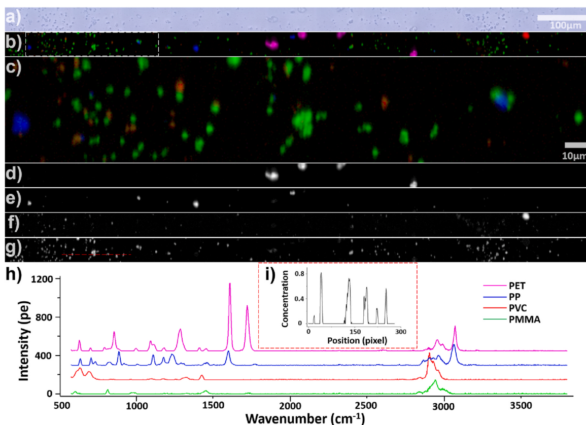
Fig. 6. Large-scale Raman imaging of a powder mixture. a) Reflection image. b) Line scan Raman component concentration image of the region in a) after FSC 3 analysis. Magenta: PET, blue: PP, red: PVC, green: PMMA. c) Enlarged image of white dashed line area in b). d)–g) Separate component concentration images of PET, PP, PVC and PMMA, respectively. h) component spectra, offset for clarity. i) Concentration of PMMA along red dashed line in g).
