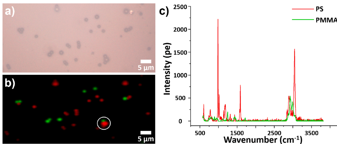
Fig. 5. Results on the 1 μm and 2 μm PS and PMMA bead mixture using the 0.6NA dry objective. (a) Reflection image. (b) Line scan Raman image of the region in (a) after FSC 3 separating the PS and PMMA chemical components, red: PS concentration, green: PMMA concentration. (c) PMMA and PS component spectra. The excitation power was 120 mW, the single step exposure time was 1 s, and the step size 350 nm.
